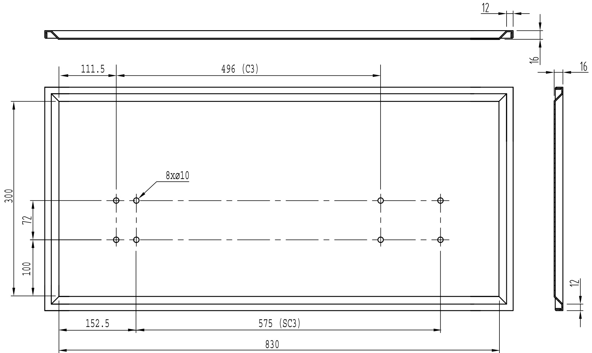
Oil Tray
